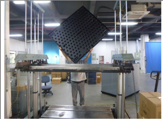
Drop test
