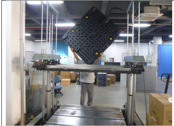
Drop test
